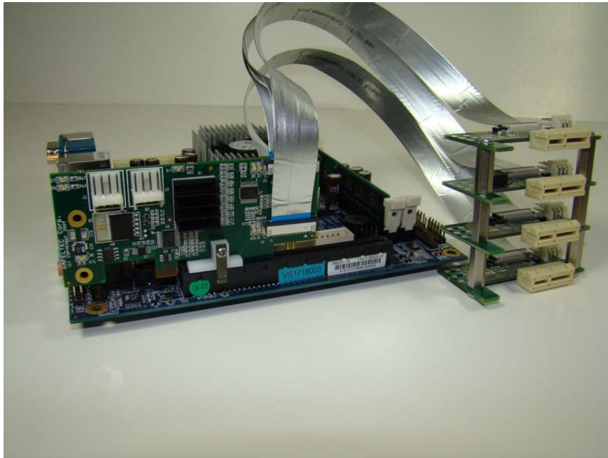
Figure 10: x1 PCI Express adapter boards in combination
