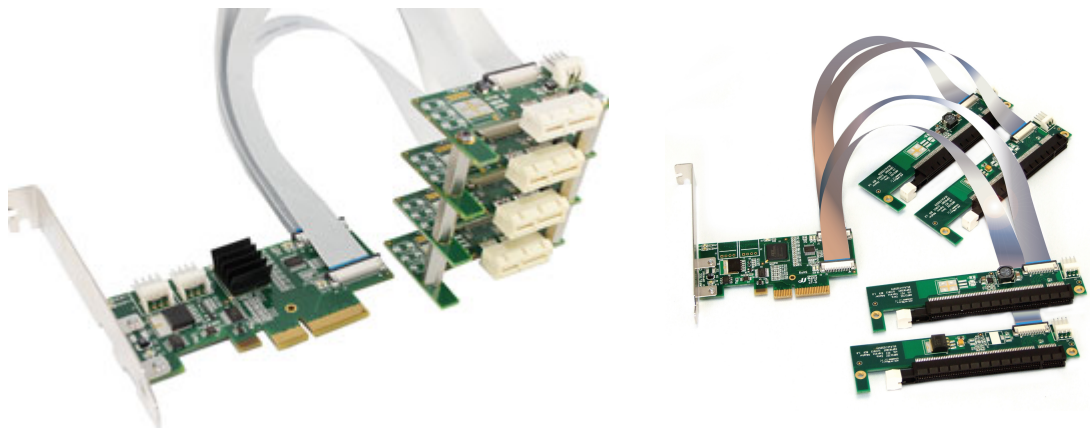
Figure 1: Flexible x4 PCI Express 4-way Splitter - x1 PCIe (left) & x16 PCIe (right) adapter board versions.
