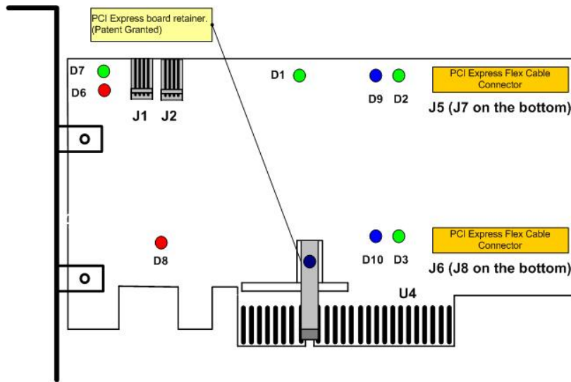
Figure 8: x4 PCI Express Host card layout
